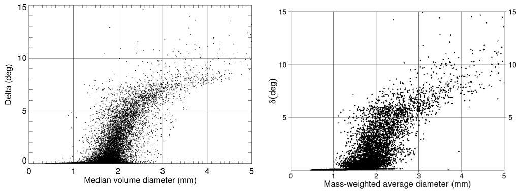
Fig. 3 The magnitude of \delta versus median volume diameter for X band and T = 20^\circ\text{C} based on DSD measurements in Oklahoma (left) and \delta versus mass-weighted average diameter for X band and T = 15^\circ\text{C} based on DSD measurements in Bonn (right).
