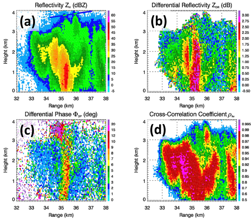
Fig. 1 Genuine RHI taken with 0.1^\circ vertical resolution using BoXPol X-band radar on 06/22/2011. Evidence of differential phase upon backscattering in a column centered at about 35 km range from the radar.
