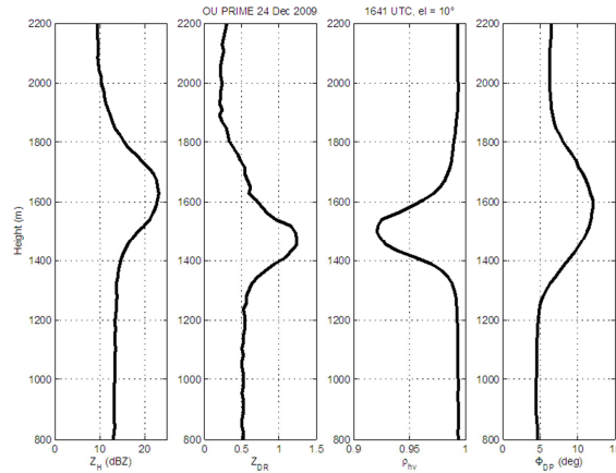
Fig. 6 Example of azimuthally averaged quasi-vertical profiles of Z_H , Z_{DR} , \rho_{HV} , and \Phi_{DP} at C band. Data are obtained on 24 December 2009, at 16:41 UTC, from the PPI at elevation 10^\circ by OU-PRIME in Norman, Oklahoma.
