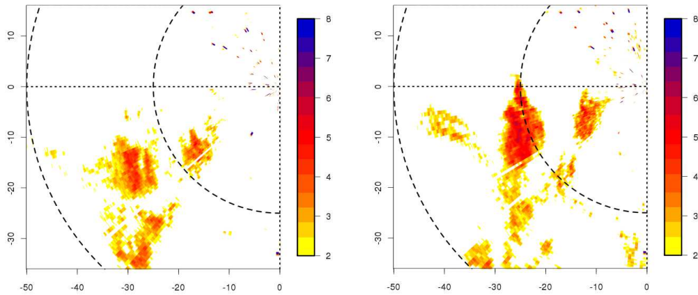
Fig. 4 PPIs of \delta generated from observations on June 22, 2011 with BoXPol in 2 consecutive time steps at 11:16 UTC and 11:21 UTC.
