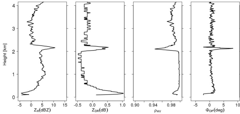
Fig. 5 Example of azimuthally averaged quasi-vertical profiles of Z_H , Z_{DR} , \rho_{HV} , and \Phi_{DP} at X band. Data are obtained on 24 September 2010, at 4:50 UTC, from the PPI at elevation 37^\circ by JuXPOL in Jülich, Germany.
