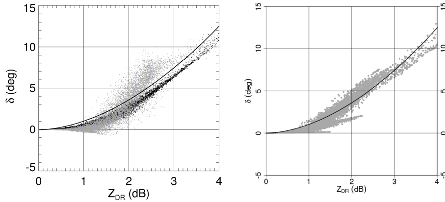
Fig. 2 Scatterplot of \delta versus Z_{DR} in rain at X band as revealed from simulations using the Oklahoma disdrometer dataset (left). Black dots correspond to temperature 0^\circ and grey dots are for temperature 30^\circ . Solid line depicts the dependence \delta = Z_{DR}^{1.8} . A similar plot but from Parsival measurements in Bonn at 15^\circ\text{C} (right) is shown for comparison.
